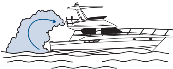
Figure 5. Engine or generator exhaust from your yacht while underway at a slow speed can cause excessive accumulation of Carbon Monoxide gas within the cabin and cockpit areas of your yacht. A tail wind can increase the accumulation. This is often referred to as the “station wagon effect”. Always provide adequate ventilation or increase your speed if possible.
